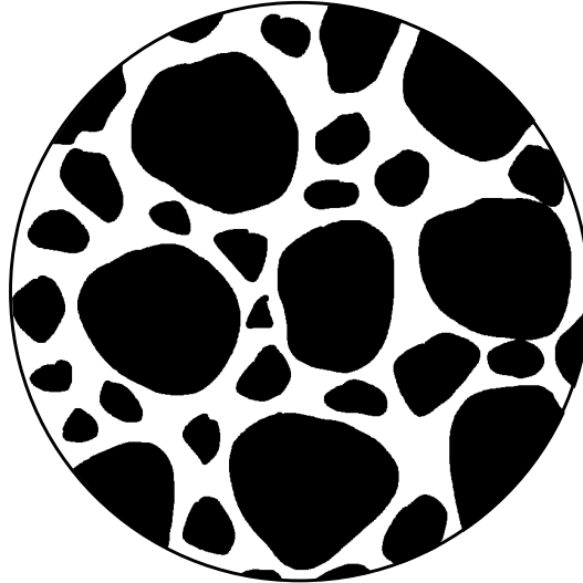
poorly sorted
