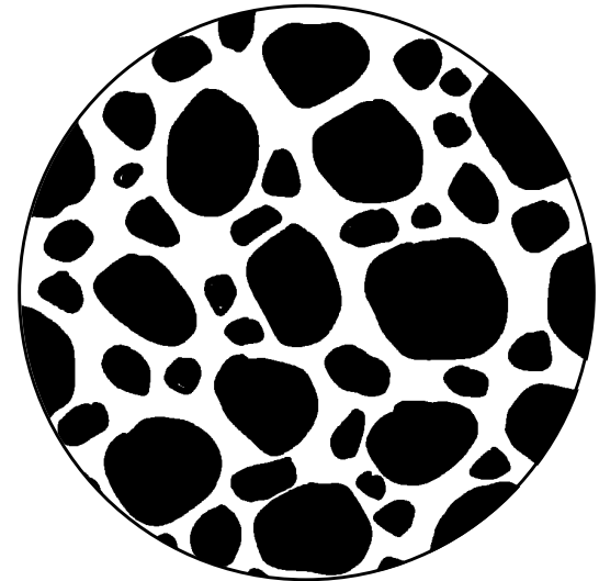
moderately sorted
