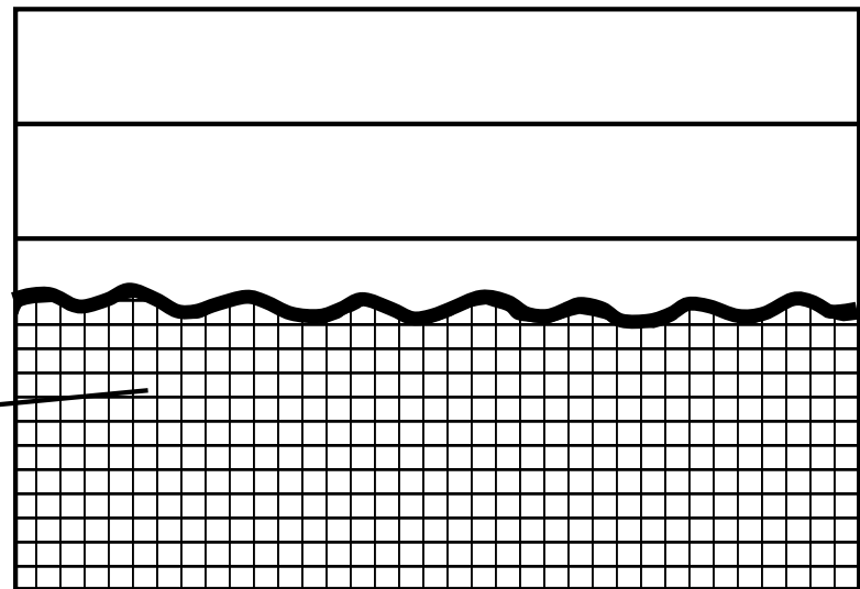
nonconformity
