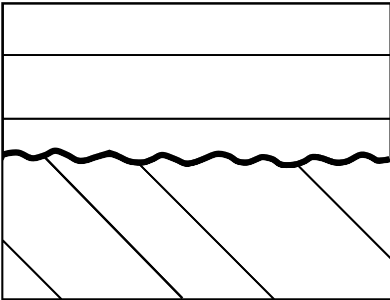
angular unconformity
