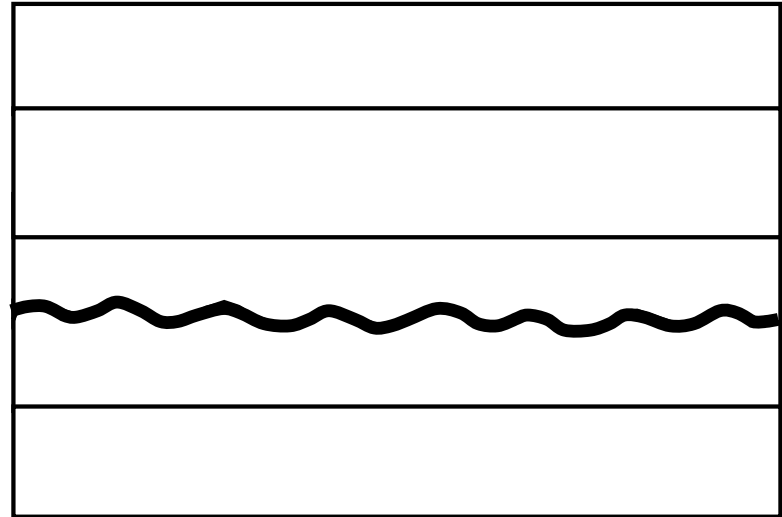
disconformity
