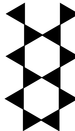
double chain
