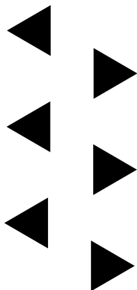
isolated tetrahedra
