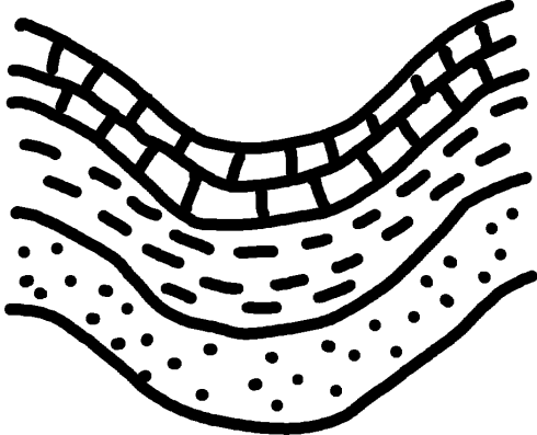
syncline
